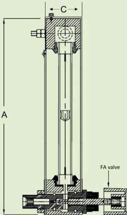
Side view of 1-way unit with FA valve
